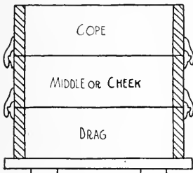
FIG. 498. THREE-PART FLASK.
